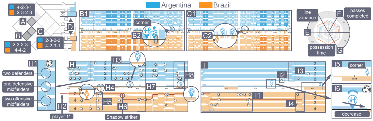
Fig. 8. Pipeline of the first case. (A), (B), (C), and (D) show the confrontation matrix. Users hover over (B) and (C) and the corresponding confrontations are shown in (B1) and (C1), respectively. (E), (F), and (G) show the statistical indicators of Argentina and Brazil. (H) shows the detail formation changes and game situations at the beginning of the second half. (I) shows the detail information of the last goal of Argentina.
