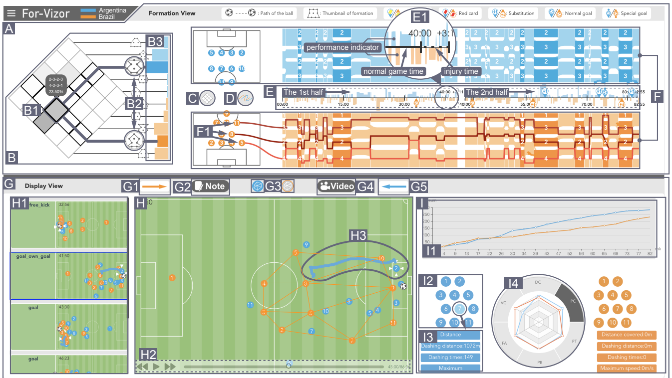
Fig. 4. System interface. The system comprises two views, namely, a formation view (A) and a display view (G). Formation view contains a confrontation matrix (B), a narrative timeline (E), and two formation flows (F). Display view contains a pitch (H) and a statistical dashboard (I).
